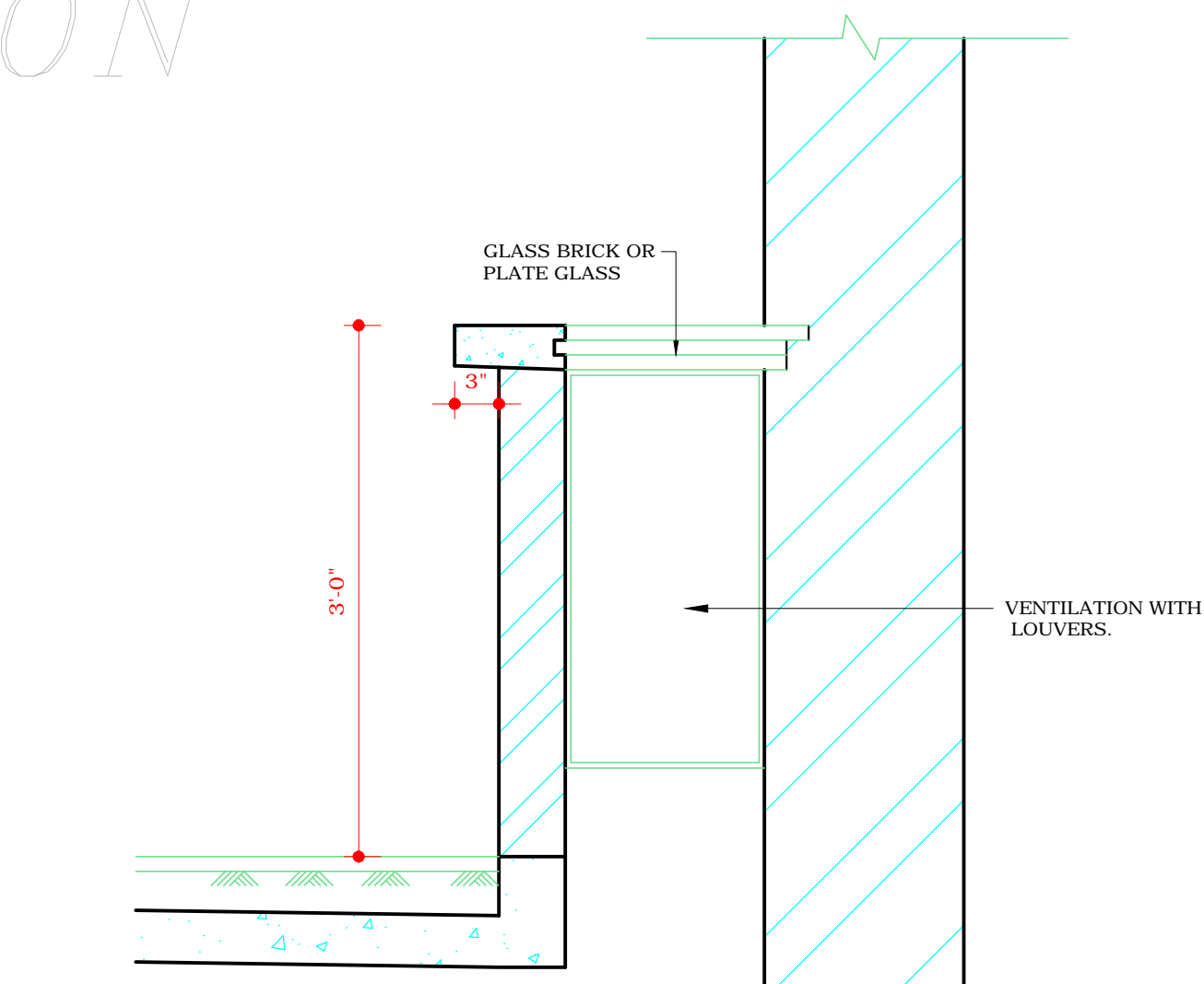
SECTION CD
