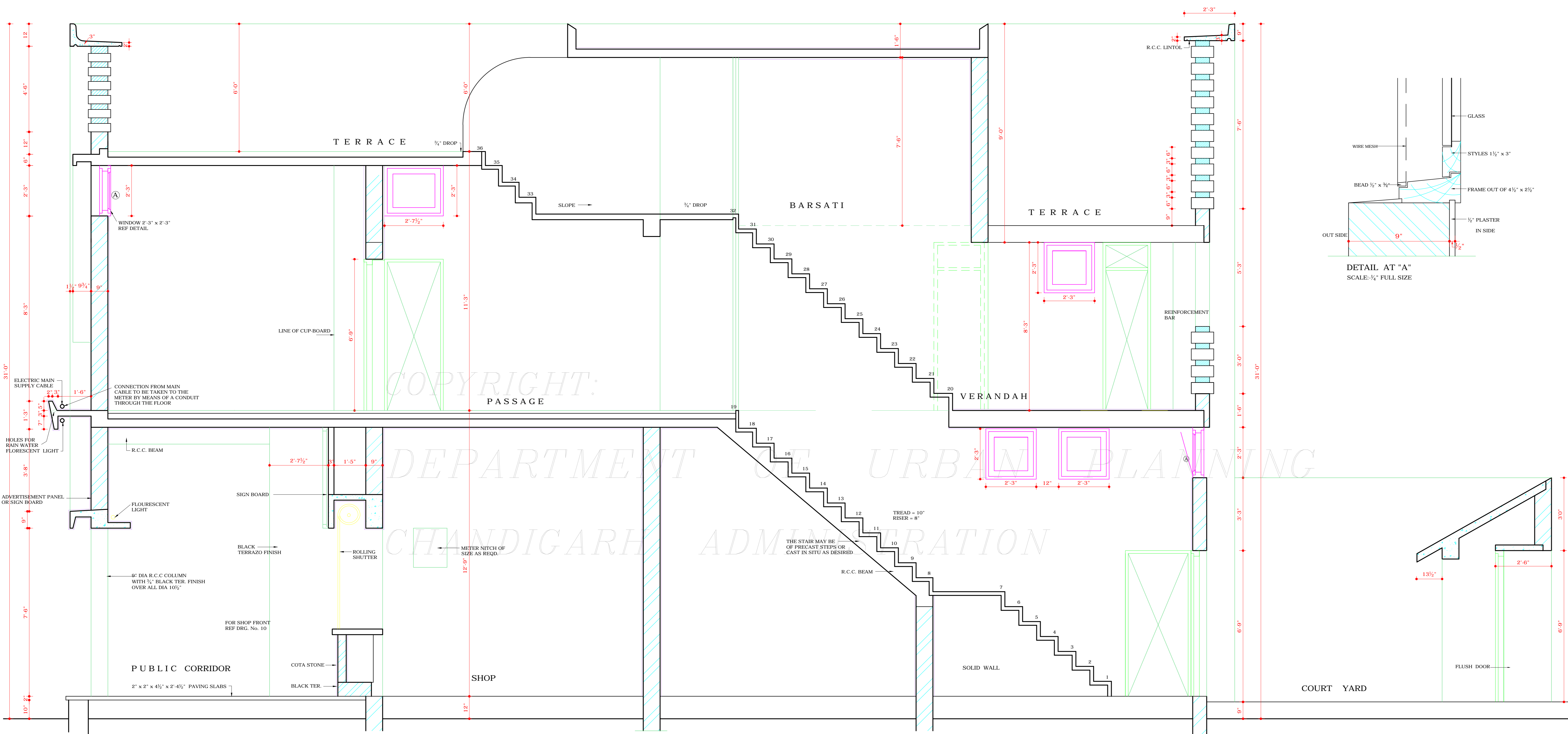
SECTION AT AA'
