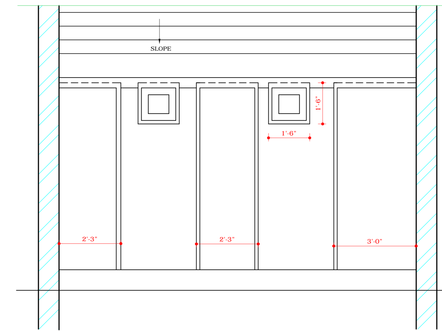
SECTIONAL ELEVATION AT CC'
