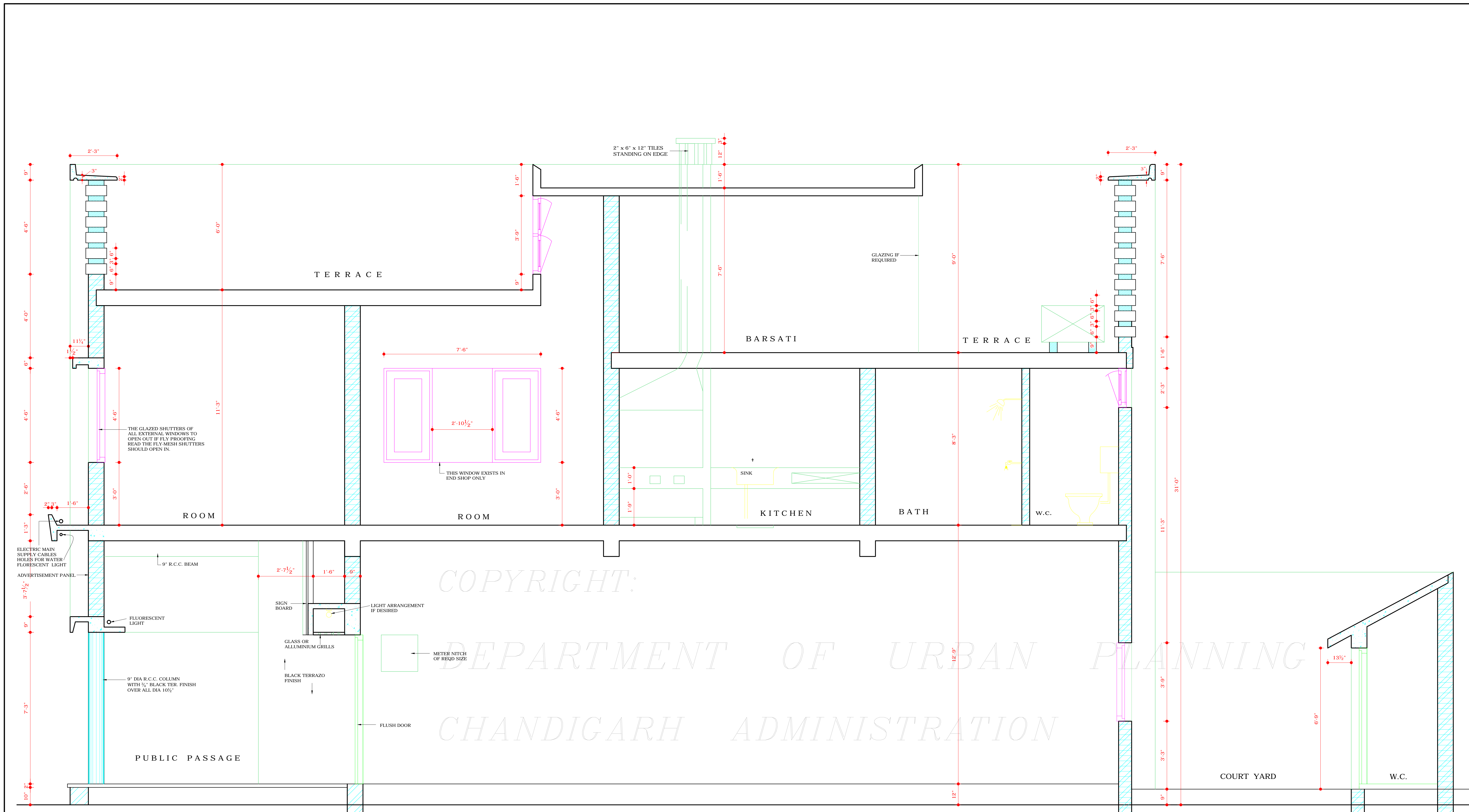
SECTION AT 'BB'
