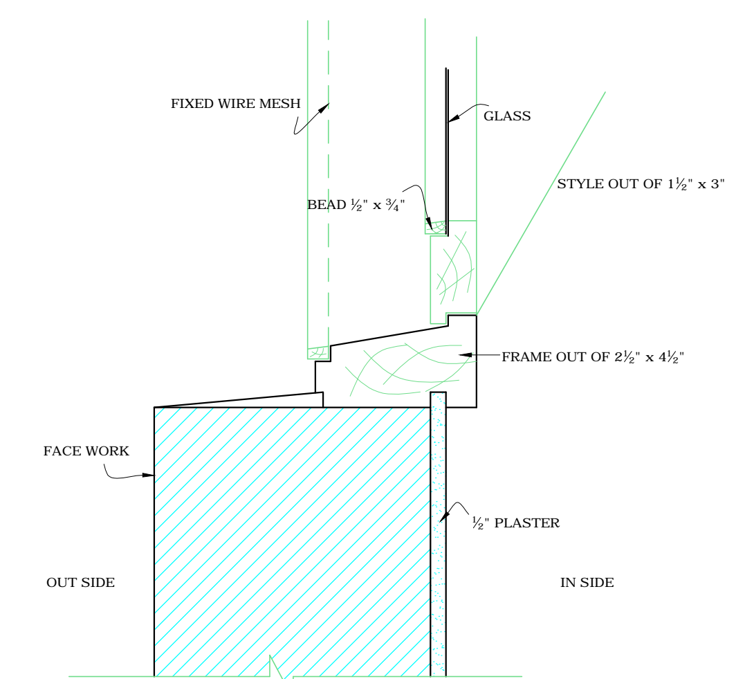
DETAIL OF B.H. WINDOW AT 'A' SCALE 1/4 FULL SIZE
