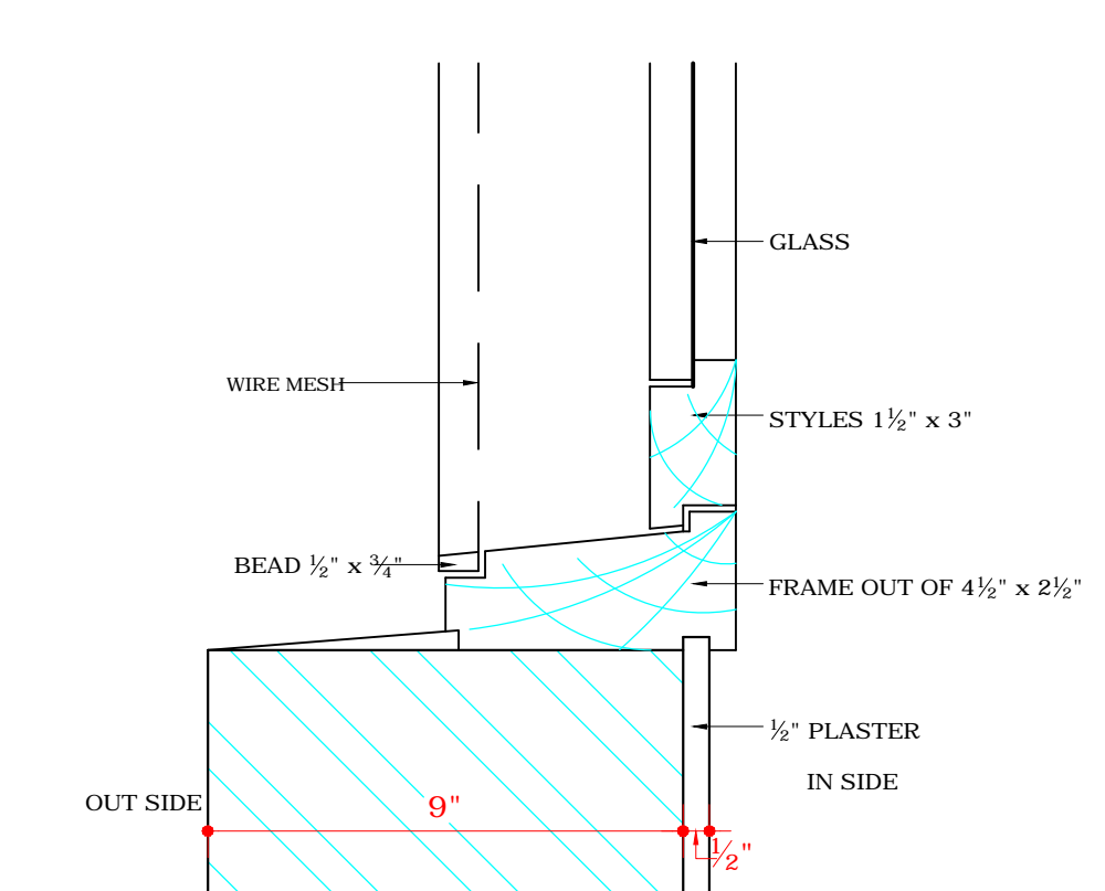
DETAIL AT "A" SCALE: 1/2" FULL SIZE
