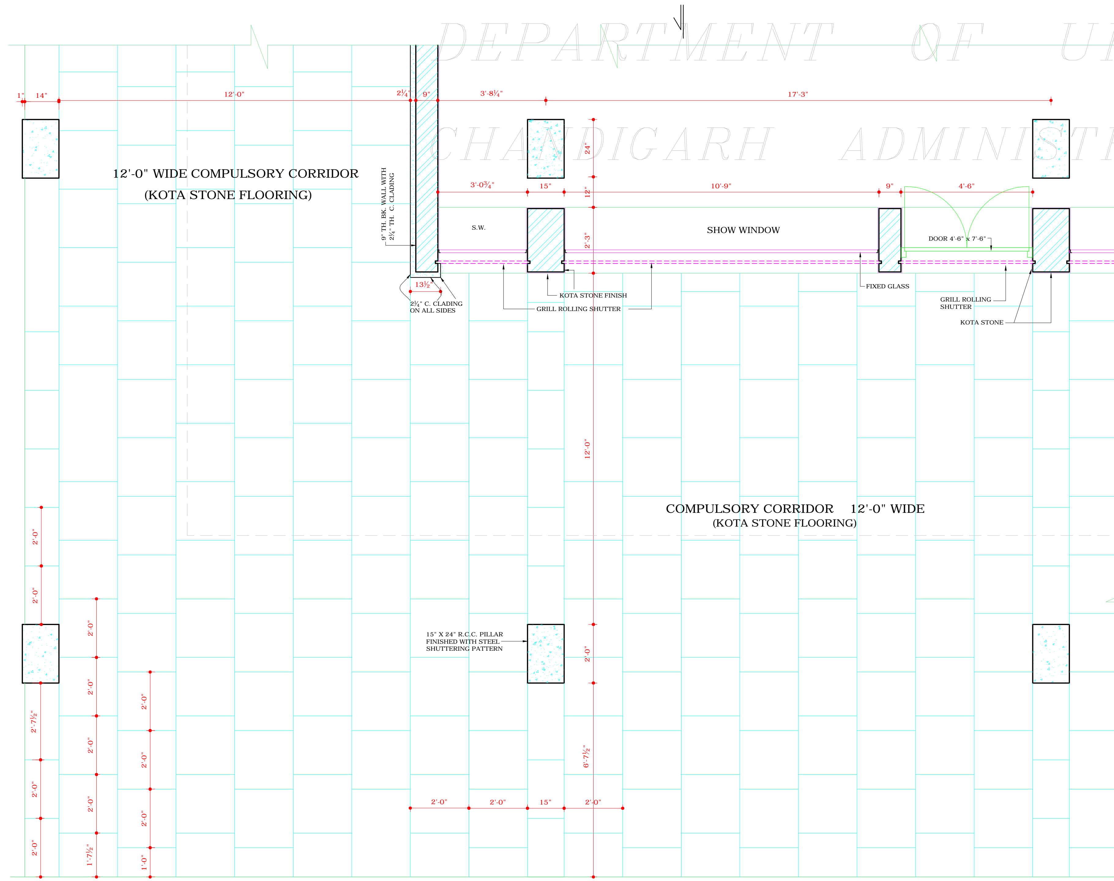
PART PLAN SHOWING SHOW WINDOW AND SHUTTERING PATTERN AT FRONT & REAR AT GROUND FLOOR
