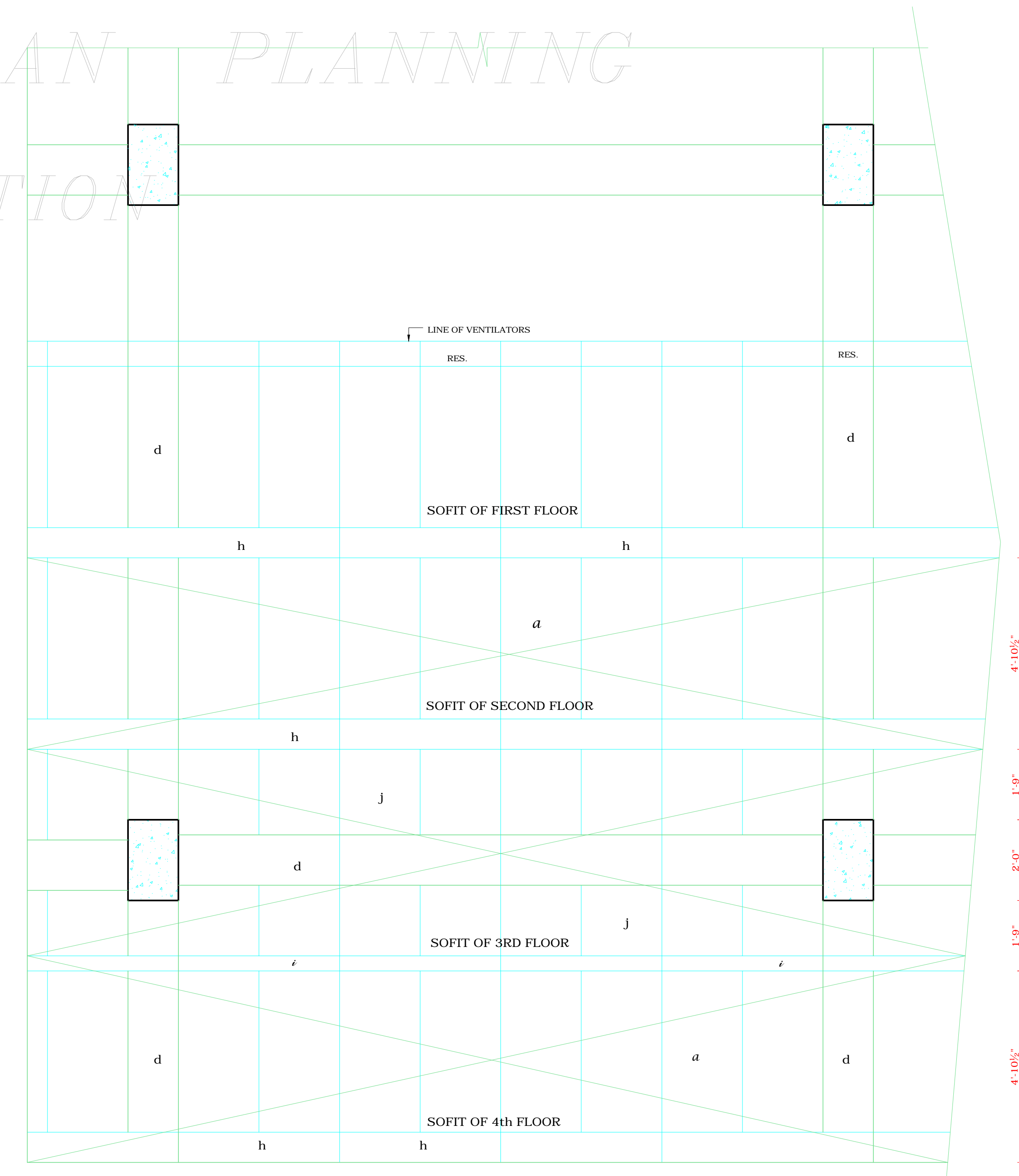
PART PLAN SHOWING SHUTTERING PATTERN ON SOFFITS OF VERANDAHS & PROJECTIONS ON FRONT & REAR
