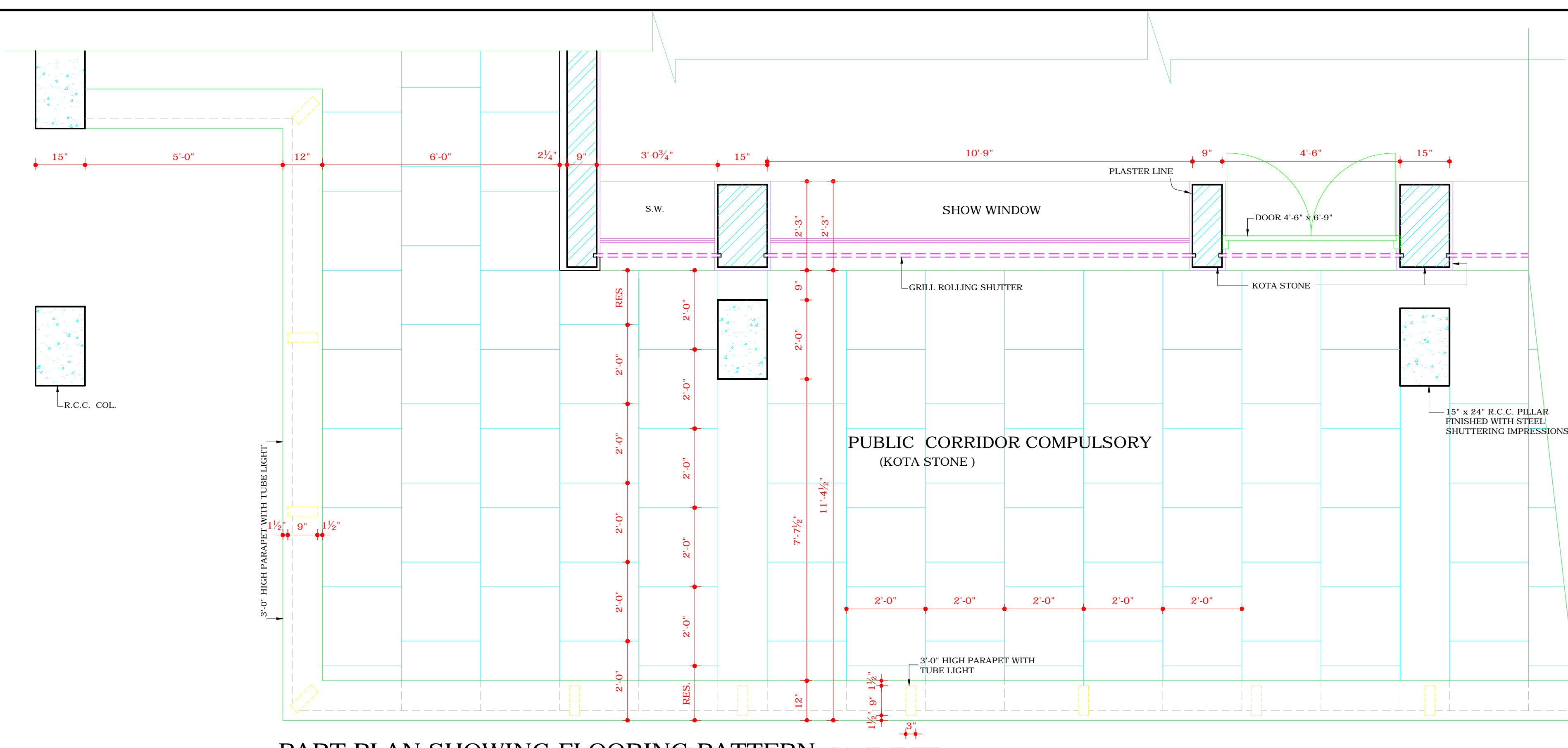
PART PLAN SHOWING FLOORING PATTERN AND SHOW - WINDOW AT FIRST FLOOR
