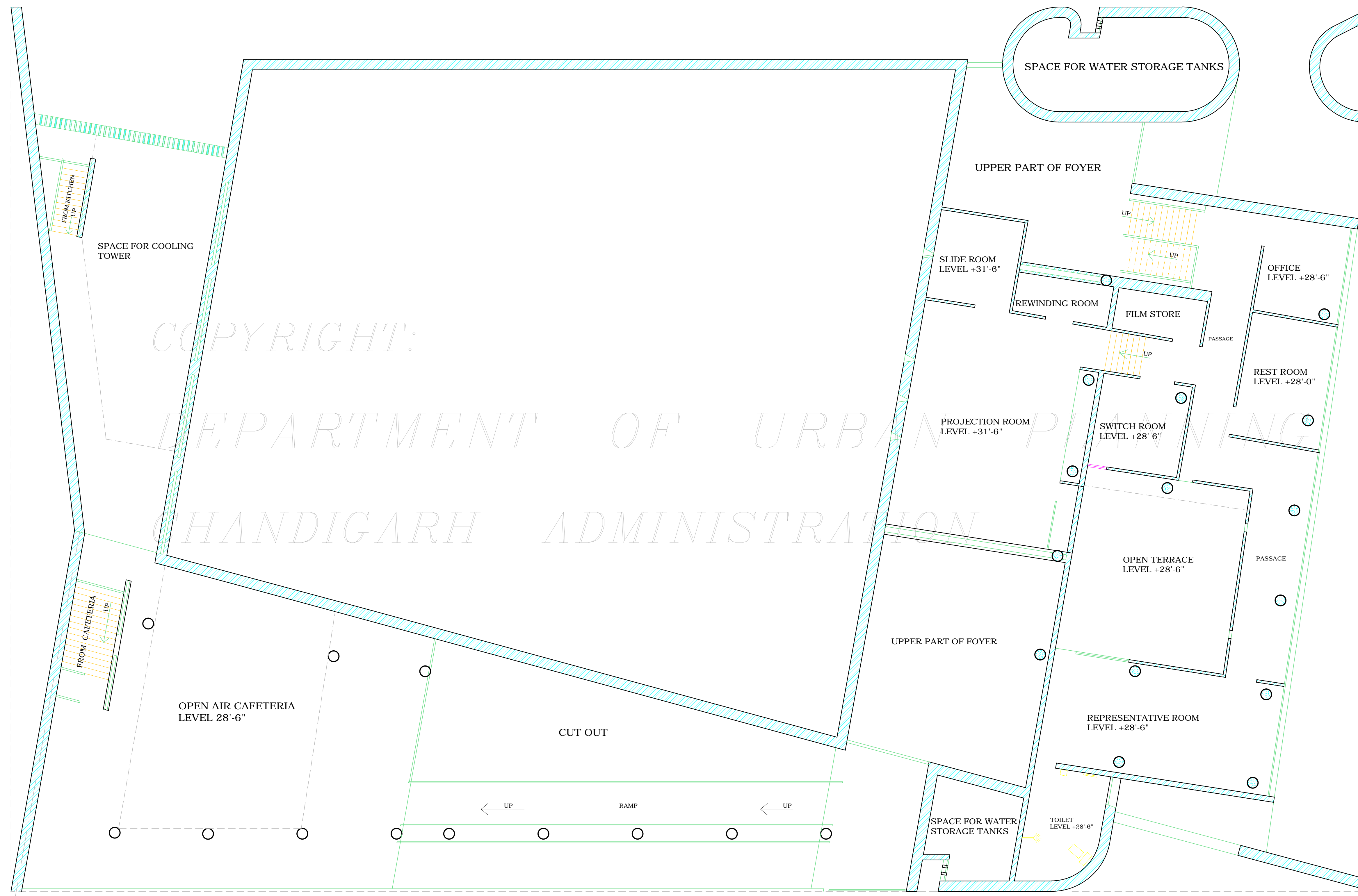
PLAN AT PROJECTION ROOM
