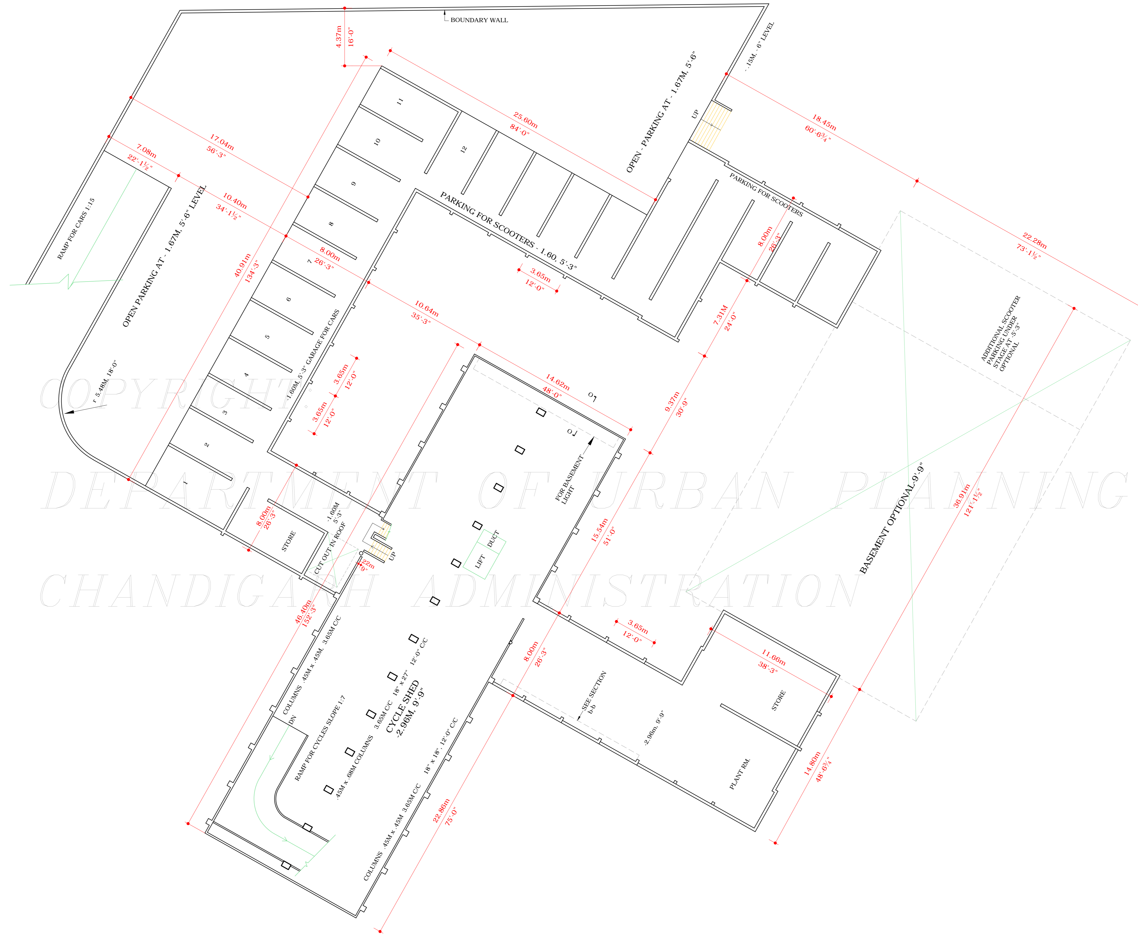
BASEMENT PLAN
