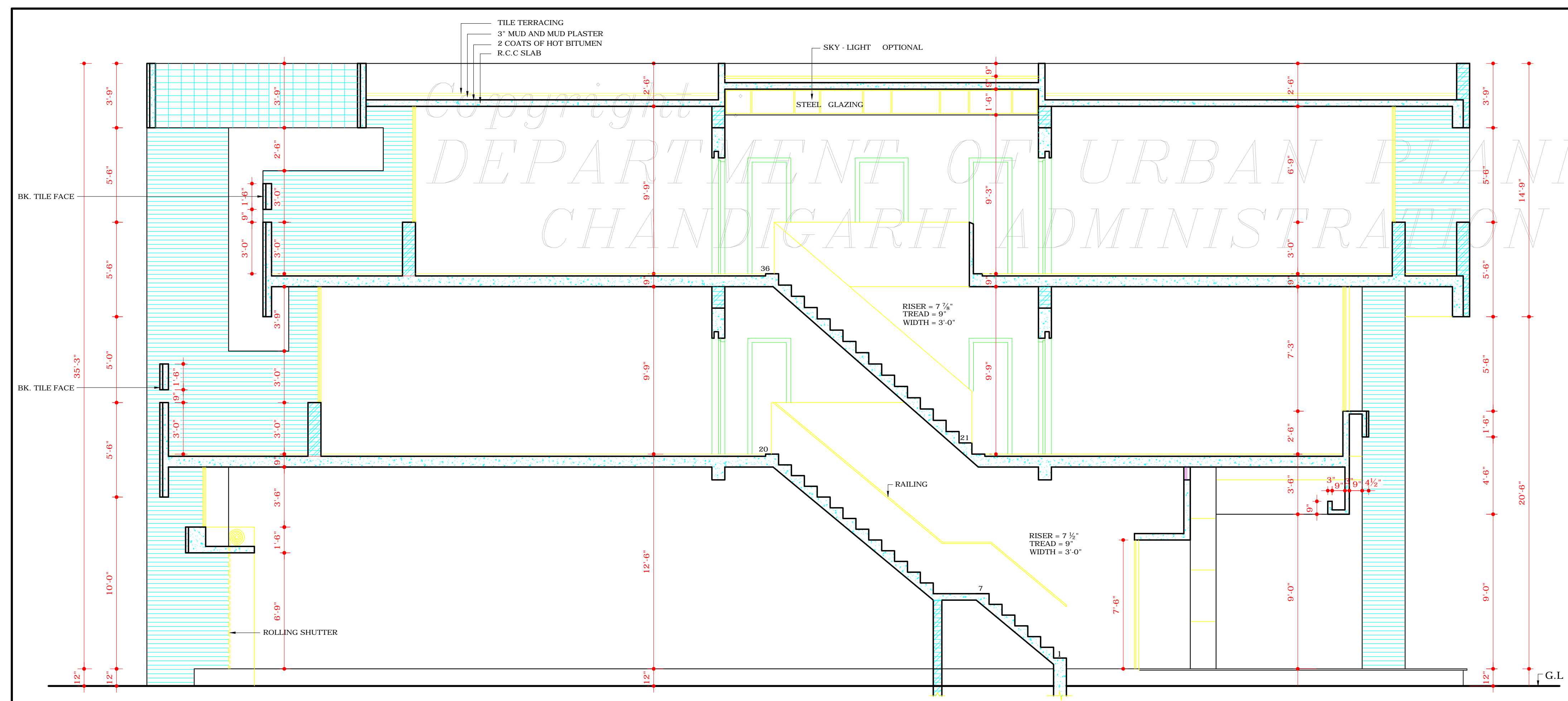
SECTION AT A-A
