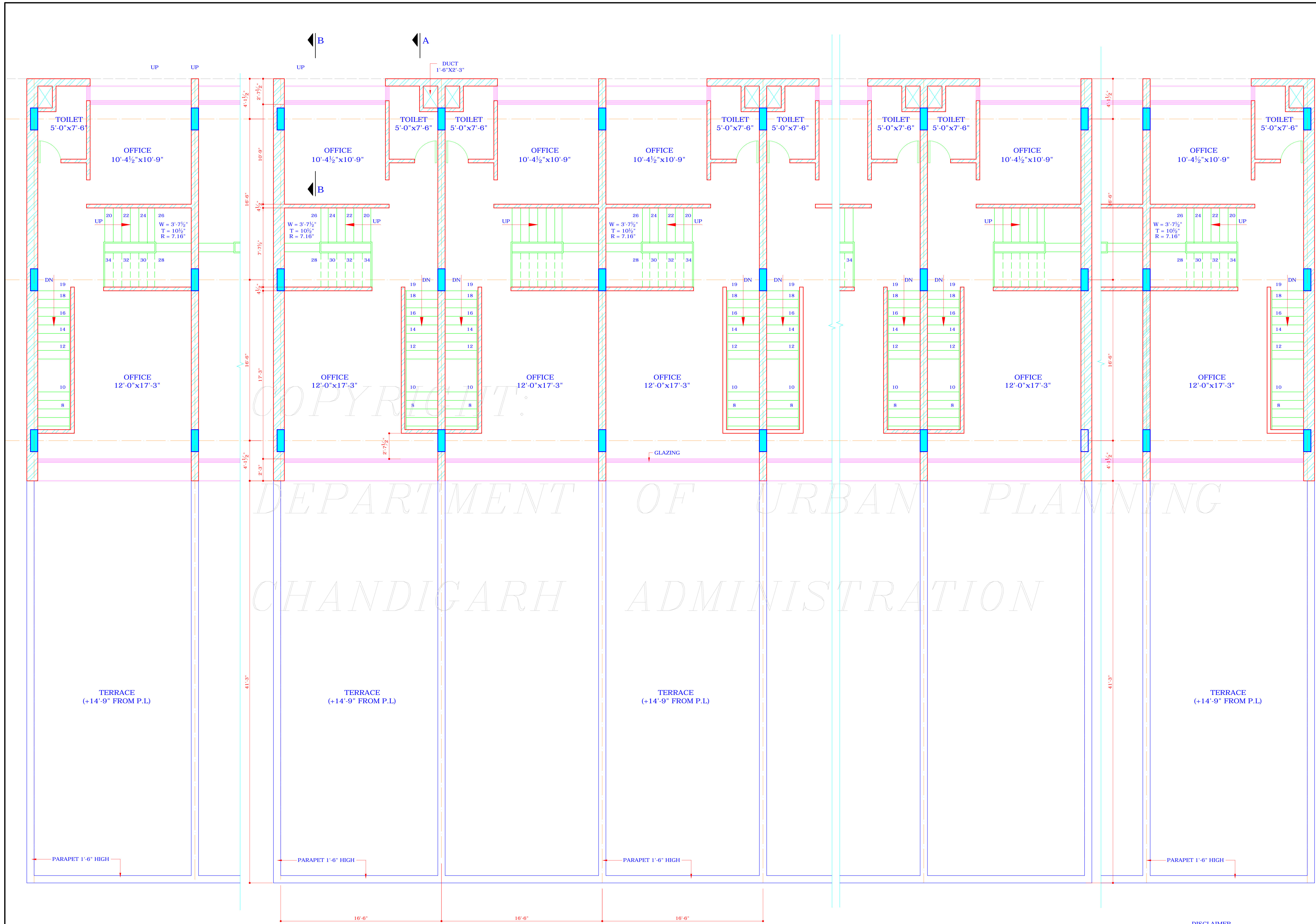
FIRST FLOOR PLAN
