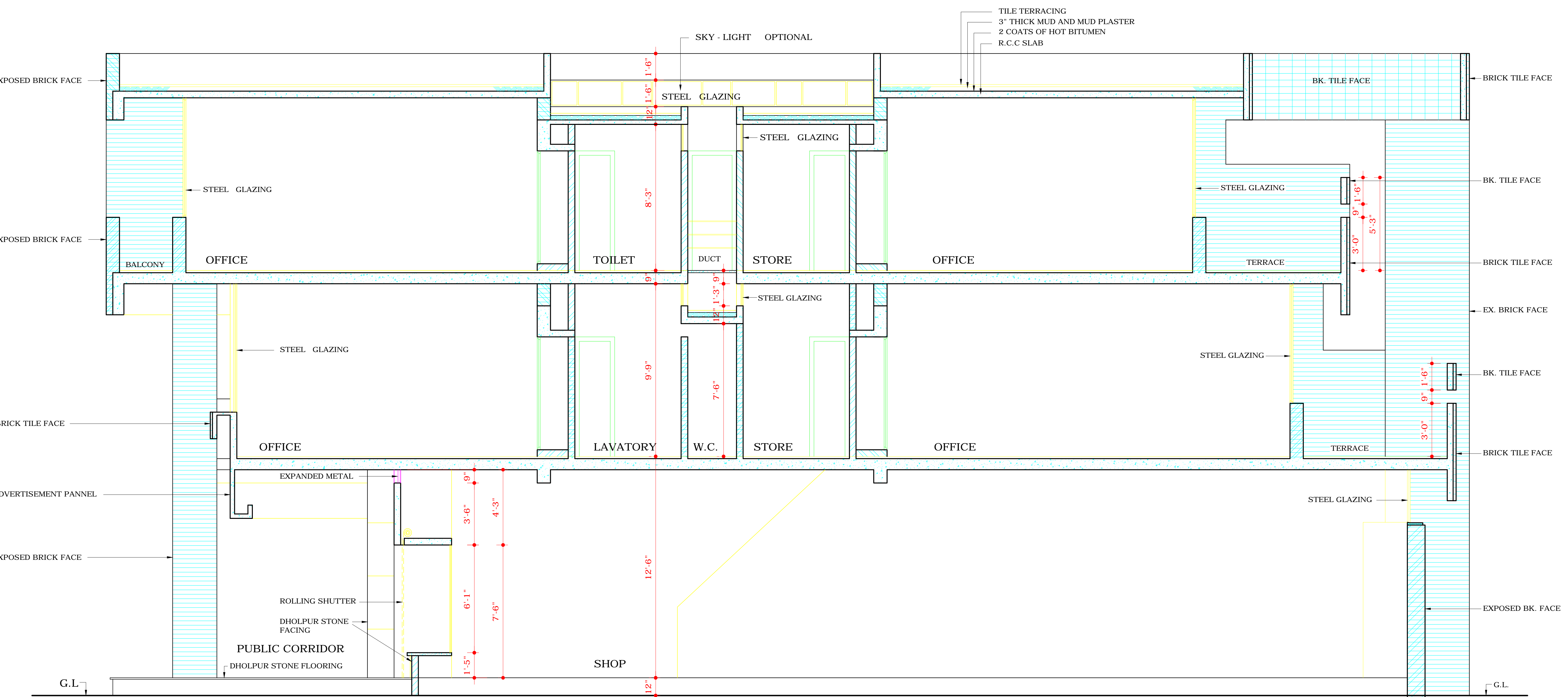
SECTION AT B-B
