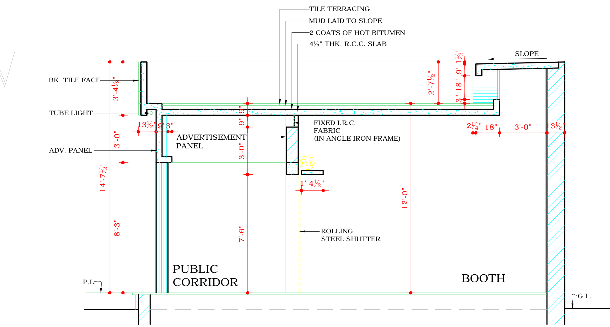
SECTION AT C - C' SCALE: 1/4" = 1'-0"
